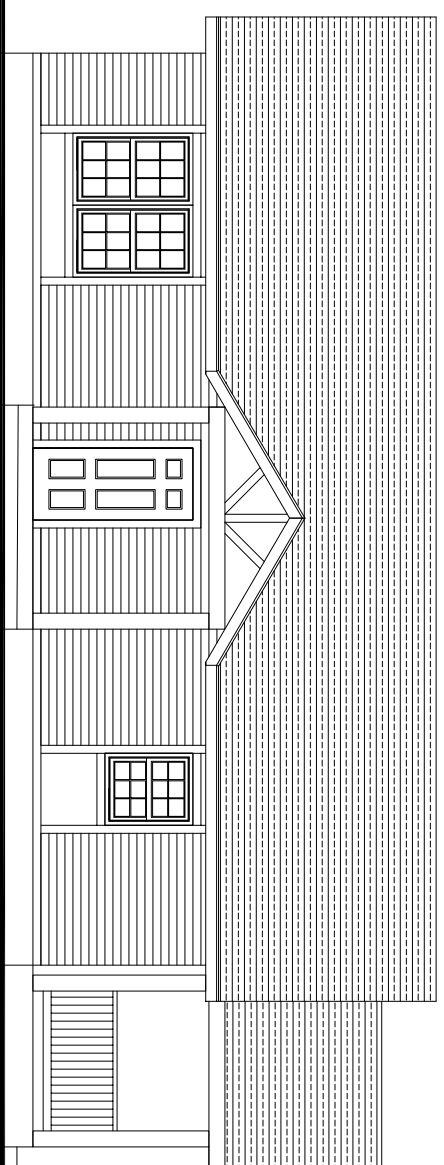
SOUTH ELEVATION
